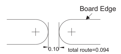
DETAIL [C] ROUTING SPECIFICATION (NOT TO SCALE)
